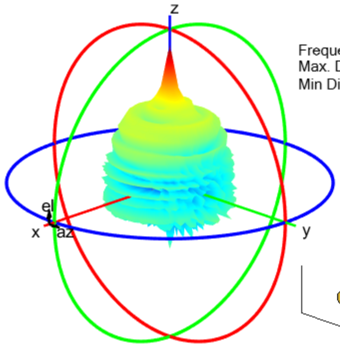
helixMultifilar
