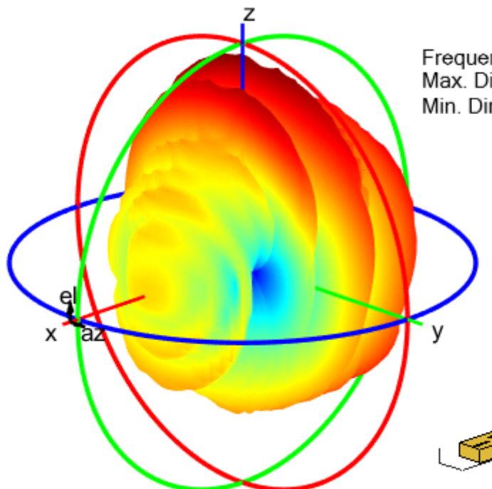
waveguideRidge
